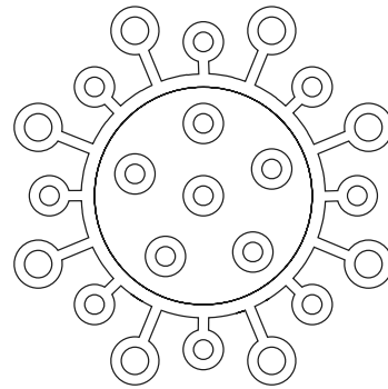
Coronavirus
