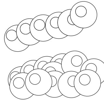
Streptococci
