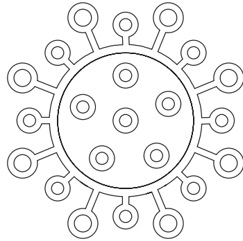
Coronavirus
