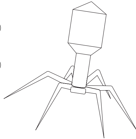
Bacteriophage
