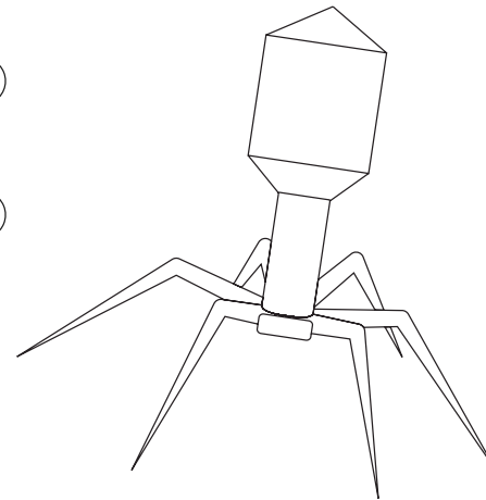
Bacteriophage
